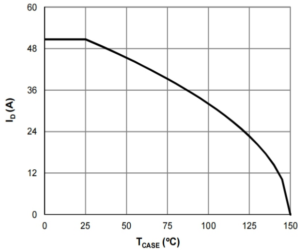
Figure 7: Current De-rating
