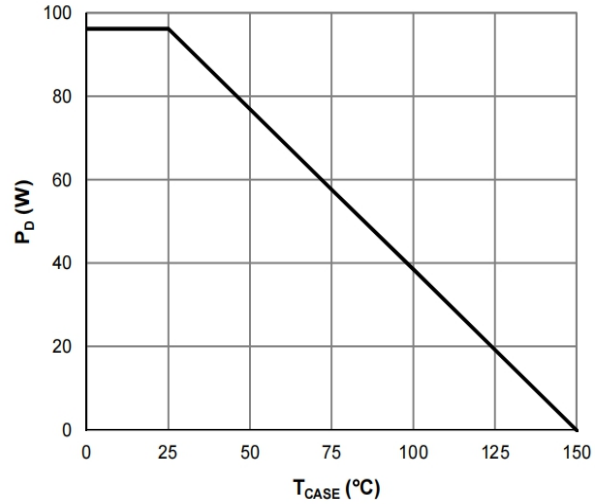
Figure 8: Power De-rating
